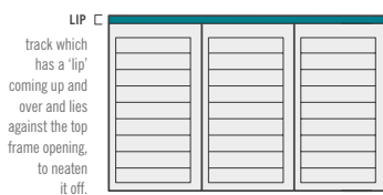
Top track with lip (To neaten uneven walls, window frames, gaps etc)
